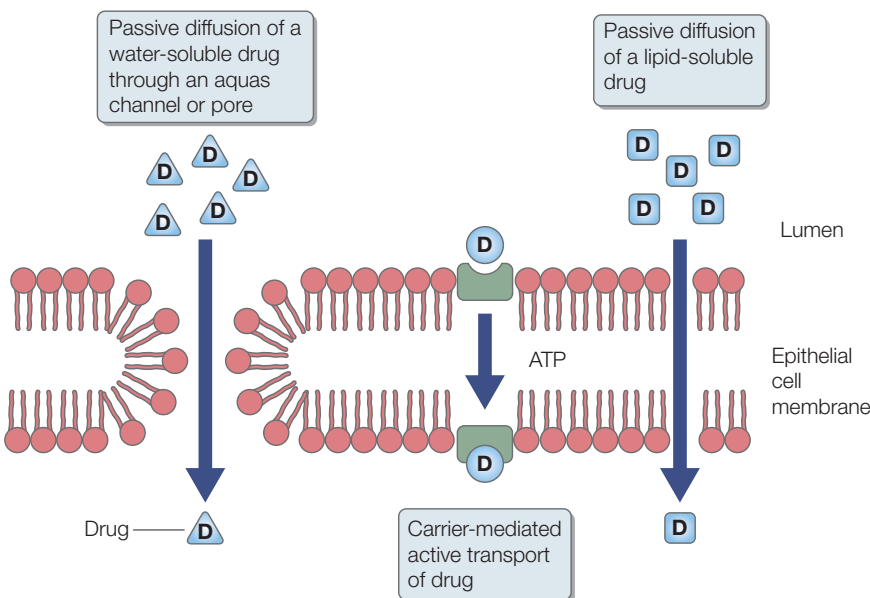
Figure 4.4: Modes of absorption of drugs from the gut.
